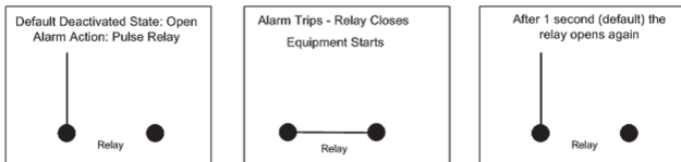
Pulse Relay
